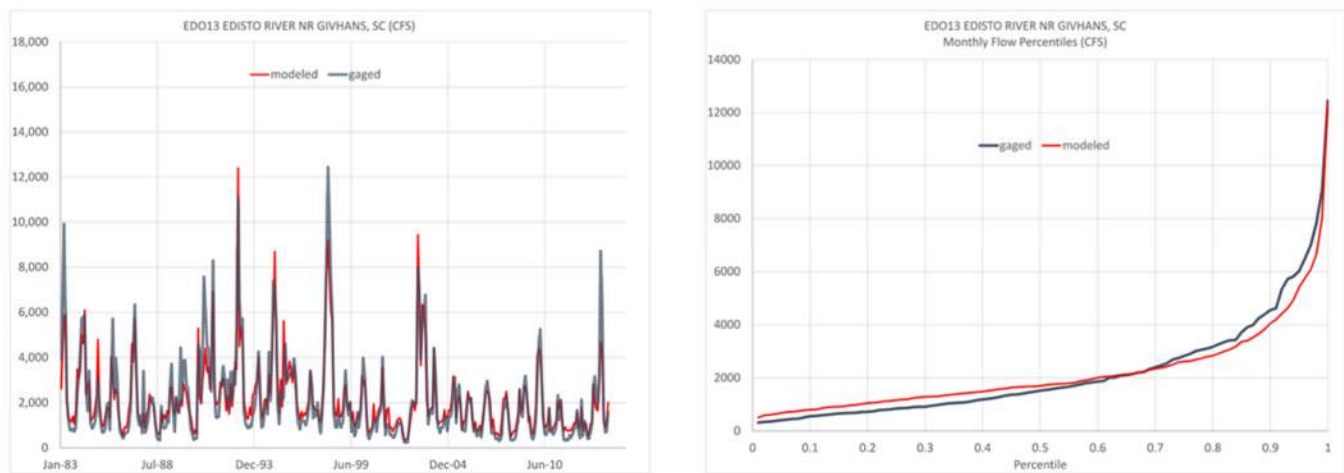
Figure 3-8. Representative Edisto River Creek basin SWAM model verification graphs (CDM Smith 2017).
