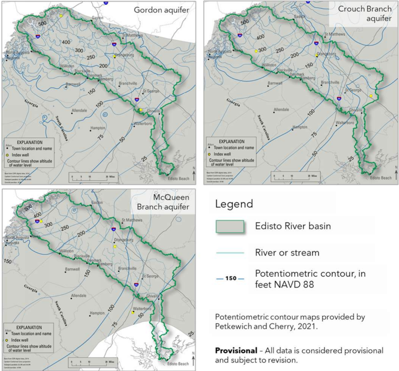
Figure 5-12. Simulated Current Scenario 2020 potentiometric contour maps for the Gordon, Crouch Branch, and McQueen Branch aquifers.
