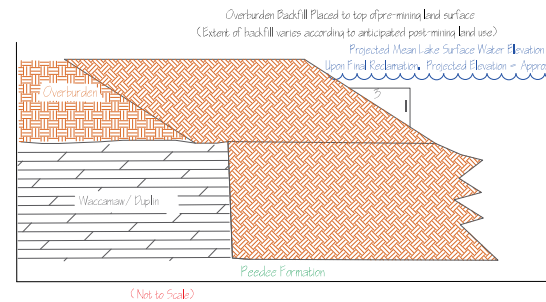
Typical Overburden Cut Slope and Pit Bench Detail Illustrating Post Reclamation Mean Lake Water Surface Elevation (Depleted Reserve area back-filled to pre-mining land surface elev.)
