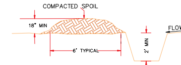
Perimeter Runoff Containment Ditch (Not to Scale)
