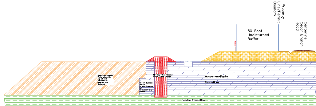
NMBQ Block A Perimeter Profile
