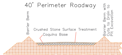
Typical 20' Perimeter Road Detail (Not to Scale)
