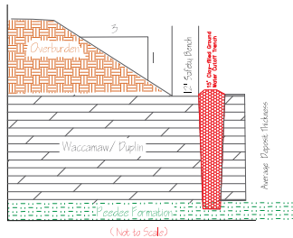
Typical Overburden Cut Slope and Pit Bench Detail (Not to Scale)
