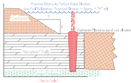
Typical Overburden Cut Slope and Pit Bench Detail Illustrating Post Reclamation Mean Lake Water Surface Elevation (Depleted Reserve area back-filled to top of rock)
