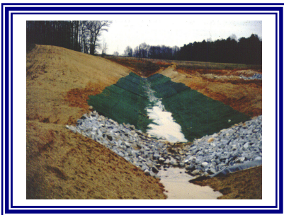
Enhanced Swales
