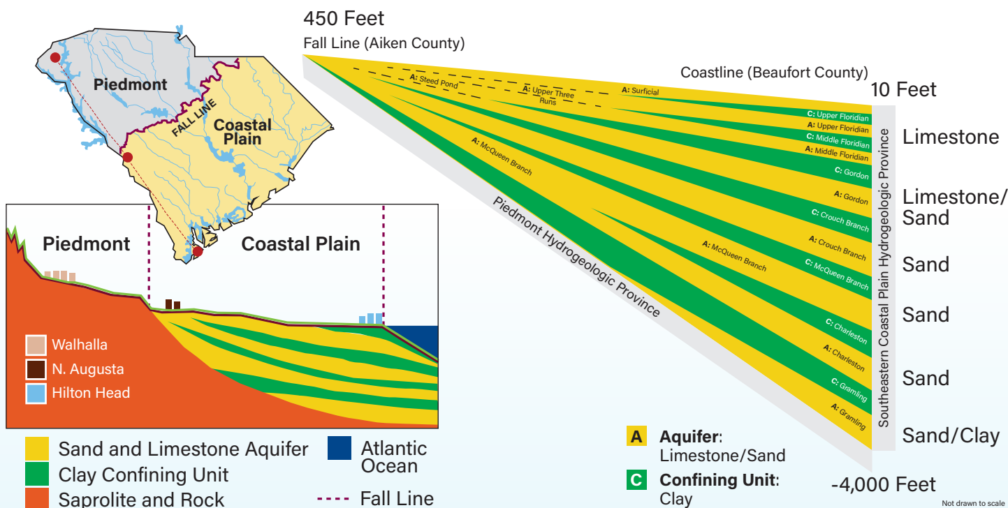
Figure ES-9. Coastal Plain aquifer system schematic cross section adapted from SCDNR 2023b.
