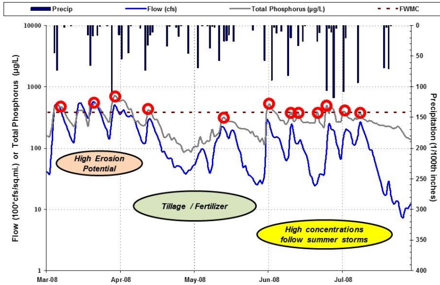
Figure 8. Maumee River total phosphorus daily patterns (March – July 2008).
