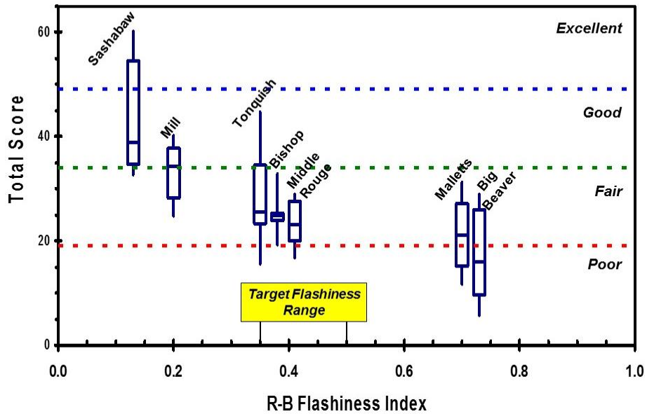
Figure 11. Comparison of stream flashiness to bioassessment scores.
