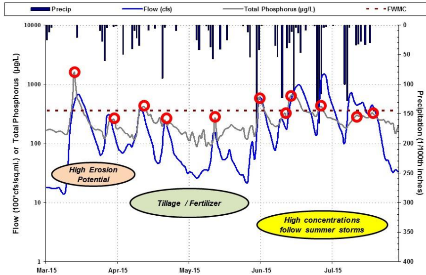
Figure 9. Maumee River total phosphorus daily patterns (March – July 2015).
