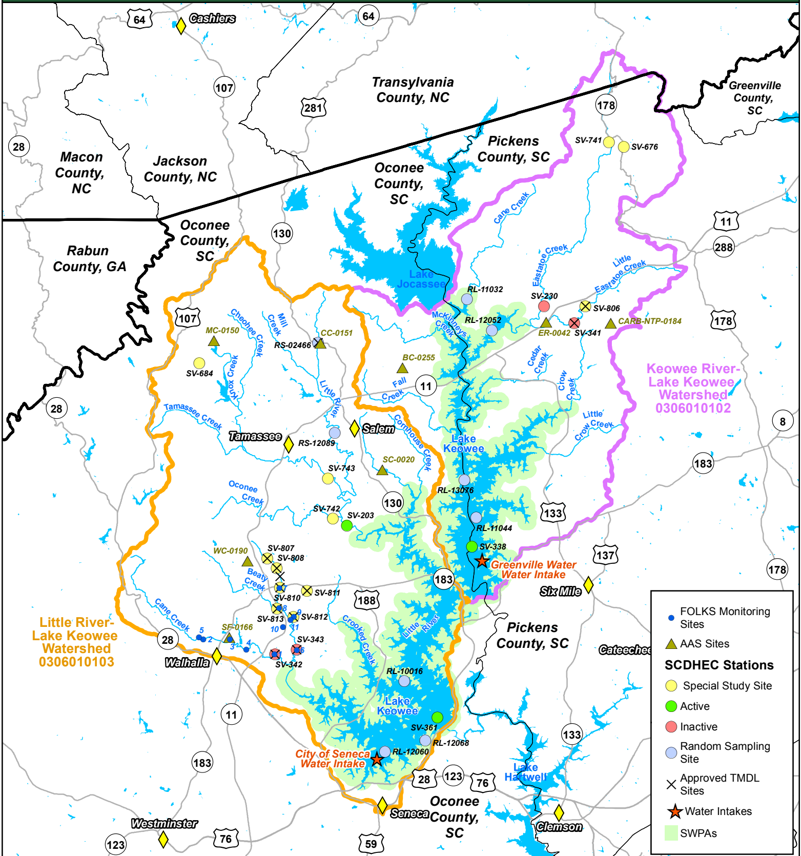
Figure 3: Monitoring Stations, Intakes, and Source Water Protection
