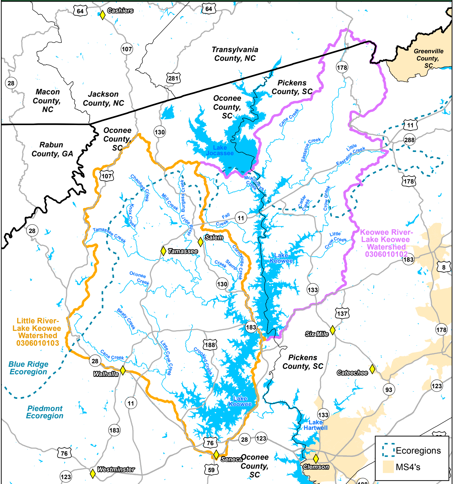
Figure 1: Lake Keowee Watersheds
