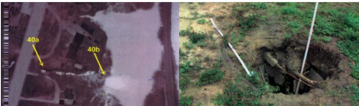
Figure 6-7: Infrared thermographic image showing septic illicit discharge (left) and the discovered cave-in responsible for the problem (Source: US EPA, 2016)
