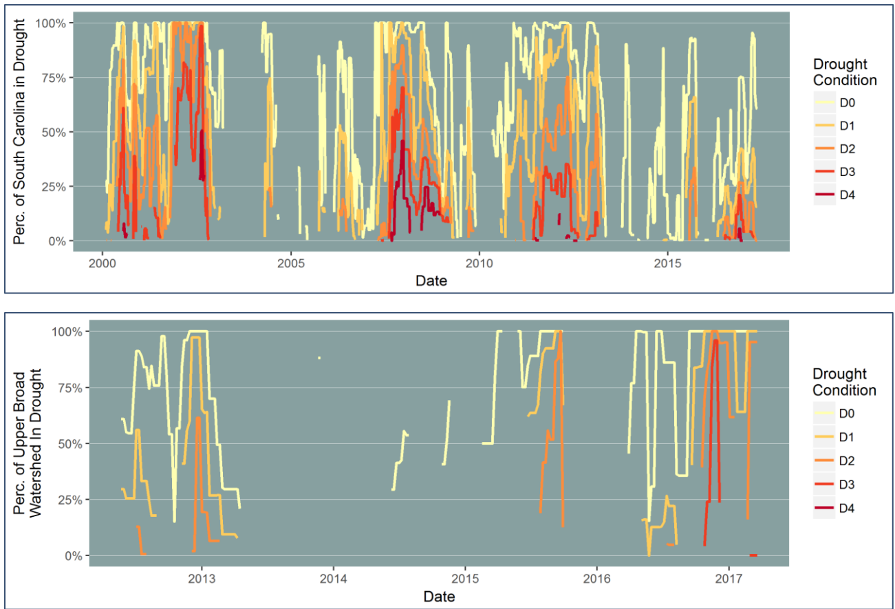
Figure 6-3: Drought Categories for South Carolina (top) and for the Upper Broad River Watershed (HUC-8, bottom)
