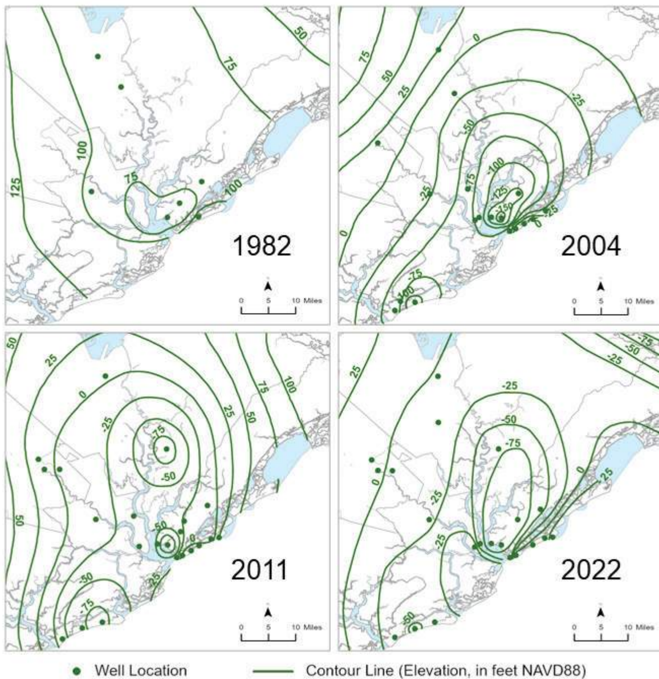
Figure 5-7. Potentiometric water level maps of the Charleston aquifer for the years 1982, 2004, 2011, and 2022. (Sources: Aucott and Speiran 1984; SCDNR 2008; SCDNR 2013; SCDNR 2023a)
