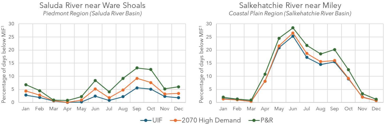
Figure 5-4. Percentage of days below MIF at two select locations.
