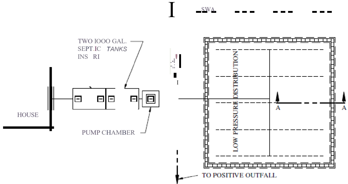
PLAN VIEW NOT 1/10 SCALE
