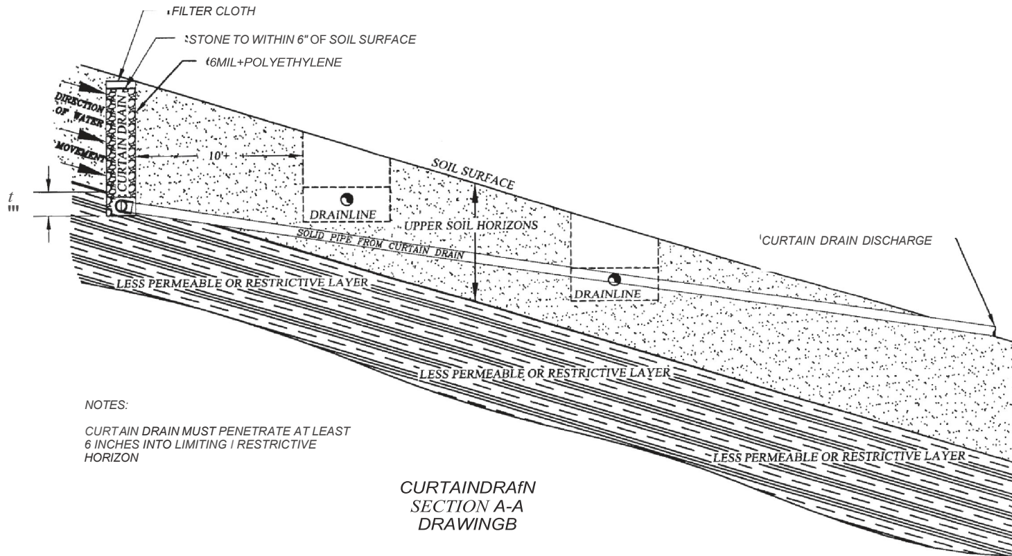
TYPICAL DESIGN SKETCH
